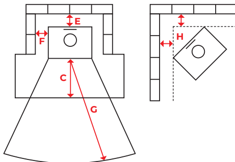
Recommended distances to non-combustibles
